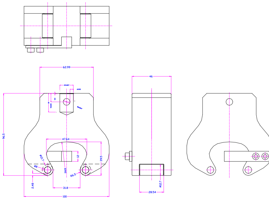
Chuck Grips per ASTM C307
