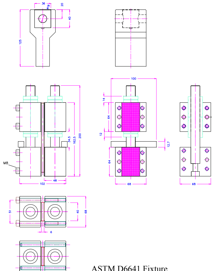
ASTM D6641 Fixture
