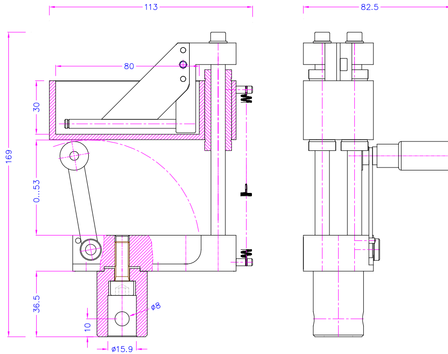
Finch Wet Device
