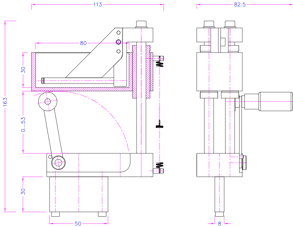
Finch Wet Device with a Sword Adapter
